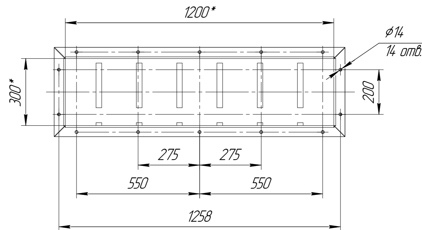
A(1:10)
